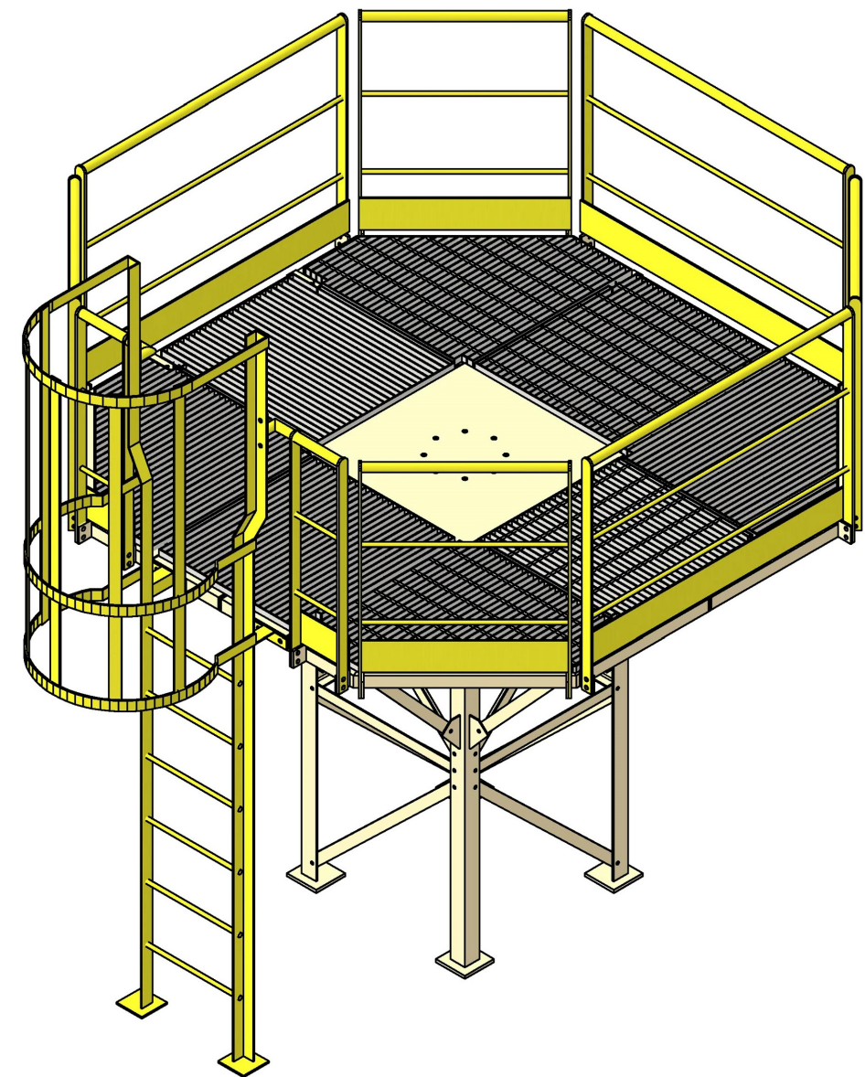
MICROWAVE ANTENNA SUPPORT MODEL
