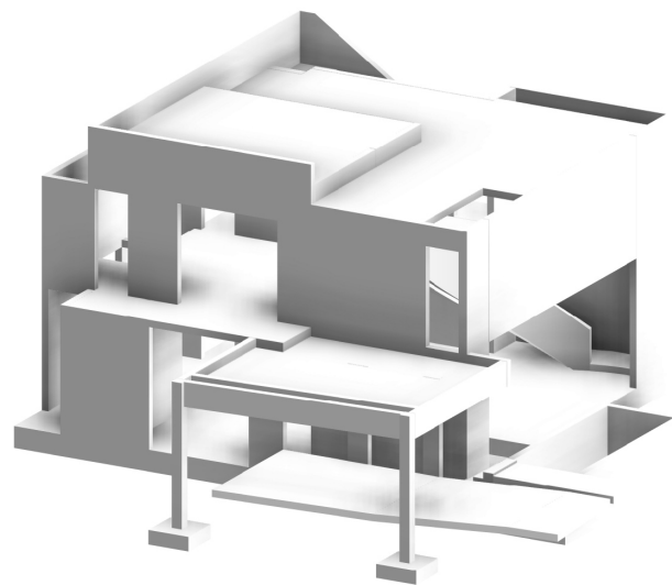
ARCHITECTURAL VIEW + PATCADS STRUCTURAL MODEL
