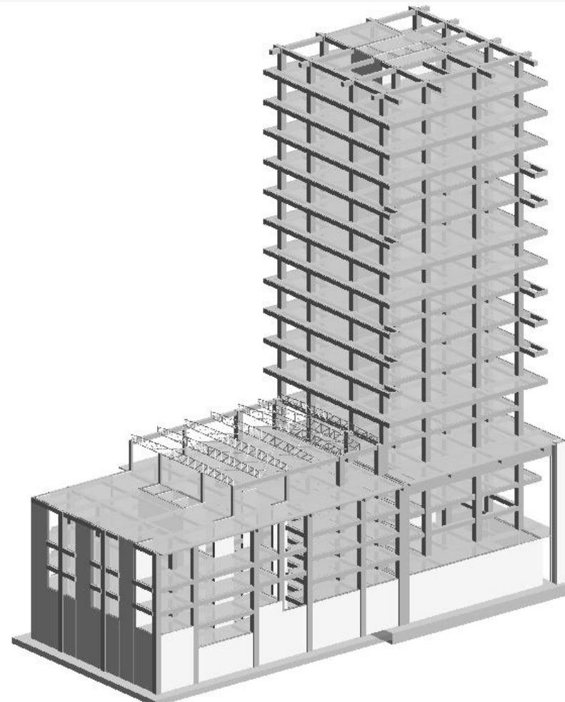
STRUCTURAL MODEL
