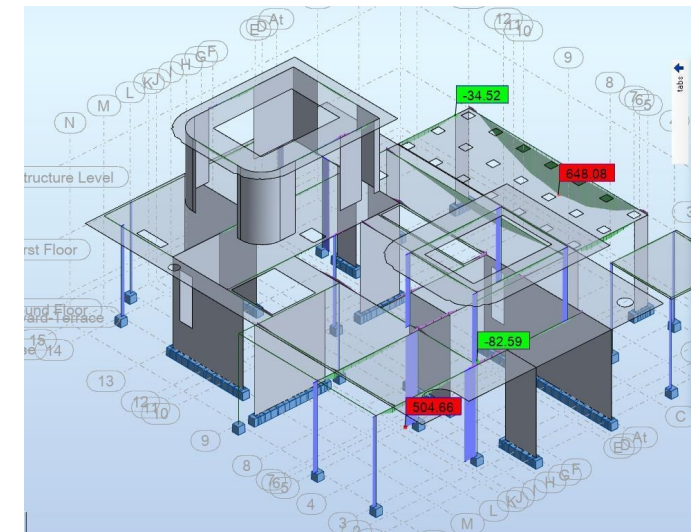
ARCHITECTURAL VIEW + STRUCTURAL ANALYSIS MODEL
