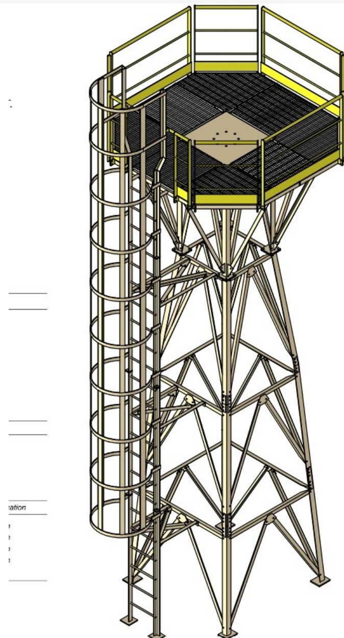
TVRO SUPPORT STRUCTURAL MODEL
